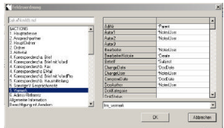
Field Mapping for a Lotus Notes Form
